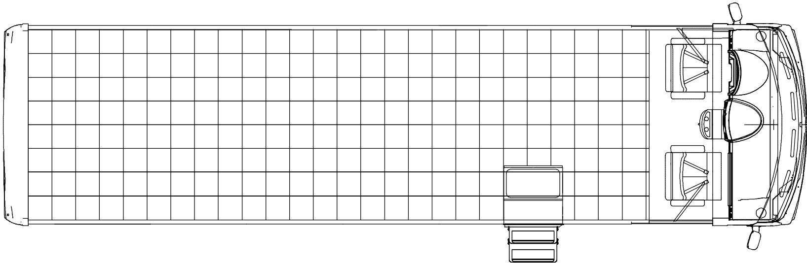
2010 WFJ33S
