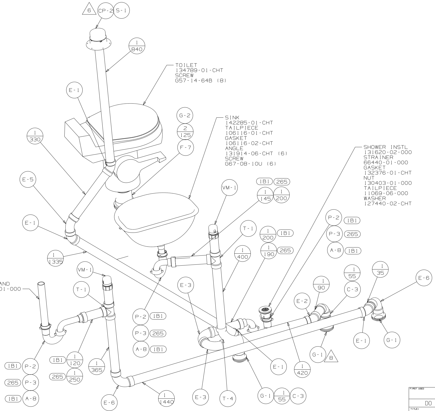
DETAIL B
