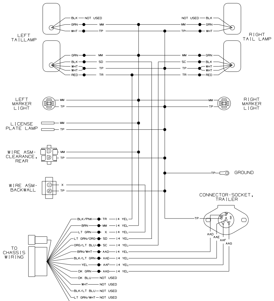
WIRING DIAGRAM-TAIL LAMPS, FD (FORD CHASSIS) (WIRE ASM 132730-01)
